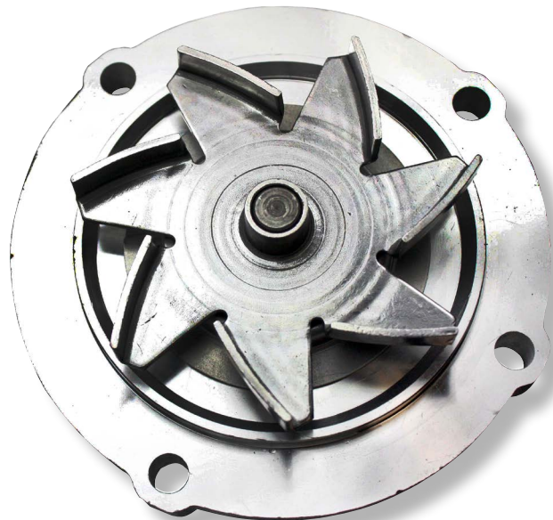
Current Design Impeller
